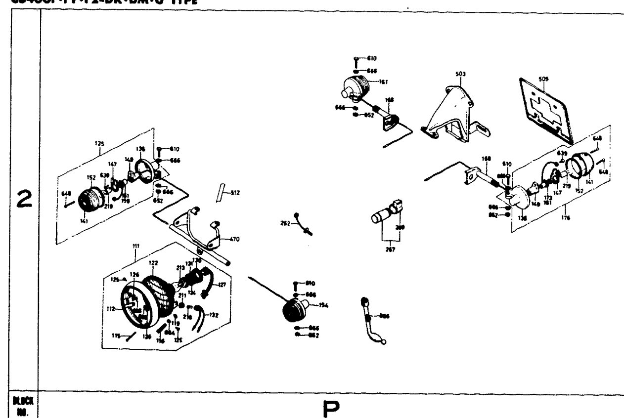
CB400F-F1-F2-DK-DM-U TYPE
