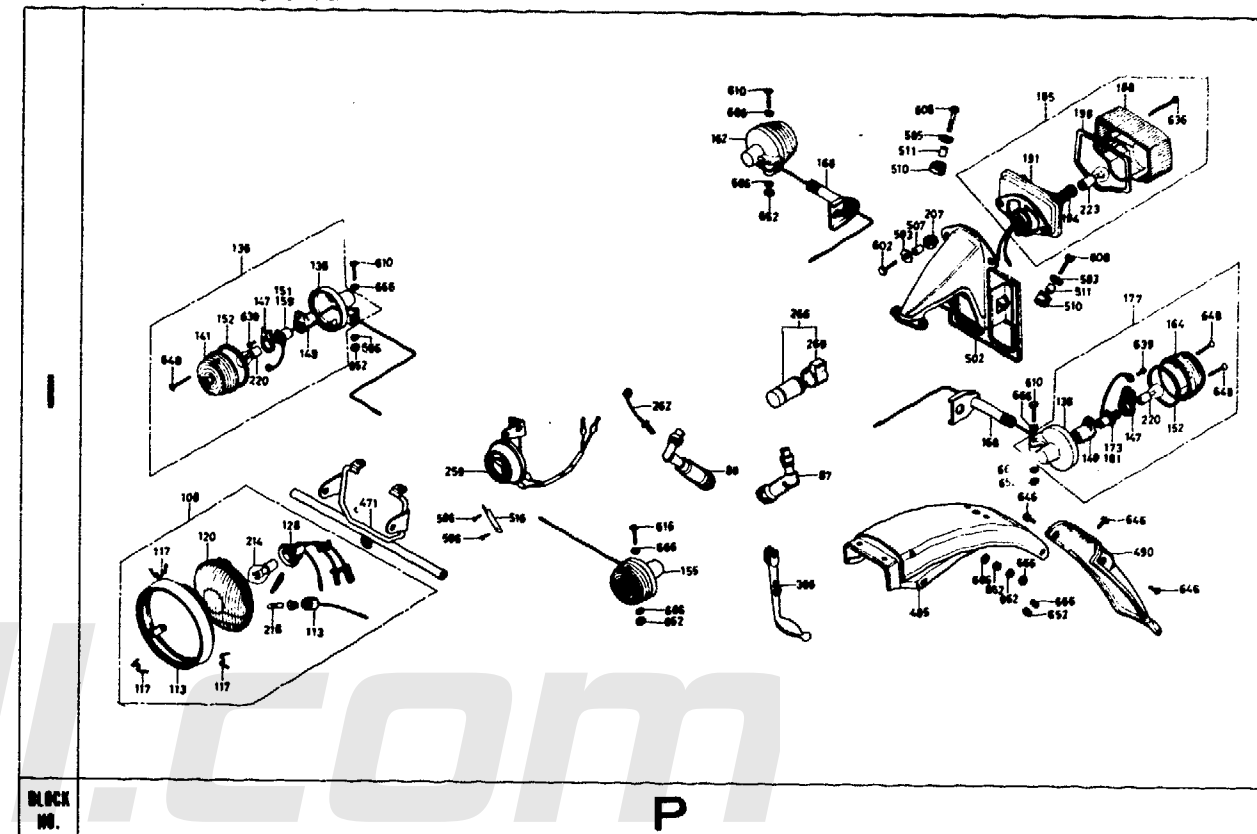
CB400F-F1-F2-DK-DM-U TYPE
