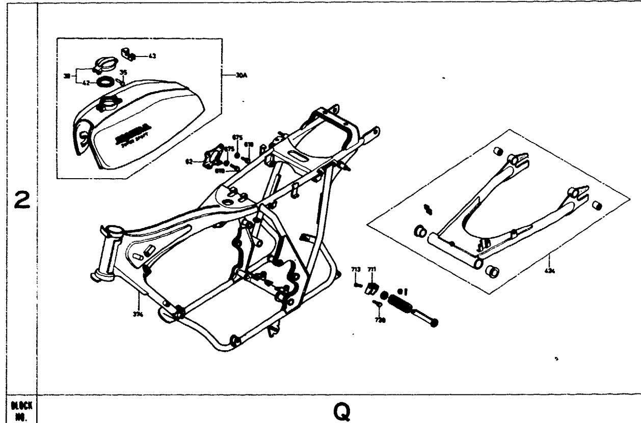
CB400F-F1-F2-E-ED-F-G-S TYPE
