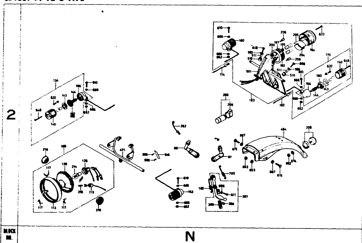
CB400F-F1-F2-G TYPE
